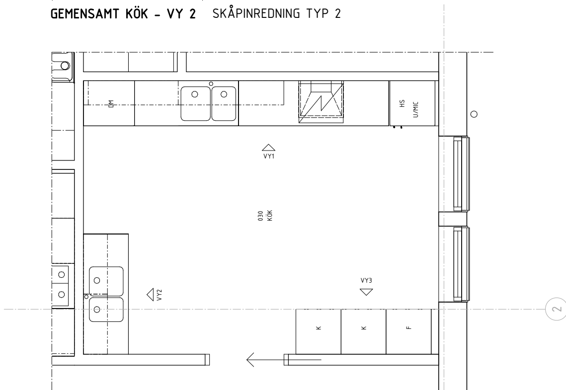
PLAN SKALA 1:25 (A3 1:50)
